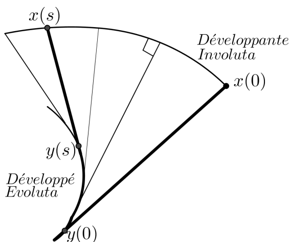
Figura 3. Evolutes i Involutes
