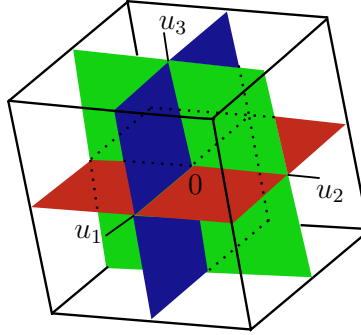
FIGURE 5. Plot of \xi_1 = \xi_2 = \xi_3 = 0 in a neighborhood of the origin. The varieties are drawn in green, blue, and red, respectively. The length of the edges of the 3d-cube is 10^{-10} .
