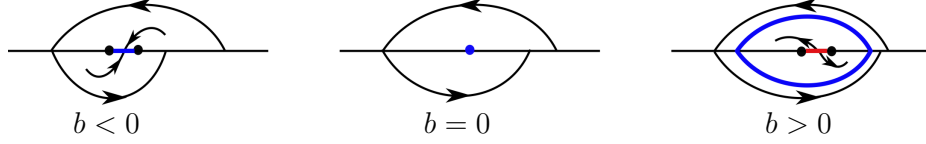
FIGURE 3. Pseudo-Hopf bifurcation.
