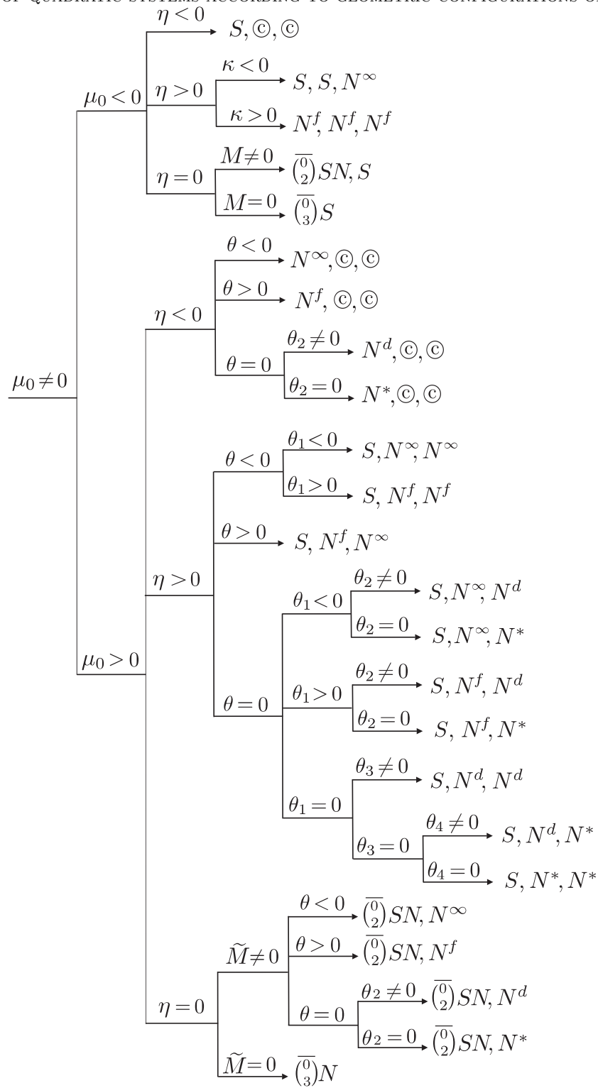
DIAGRAM 3. Configurations of infinite singularities: the case \mu_0 \neq 0 .
