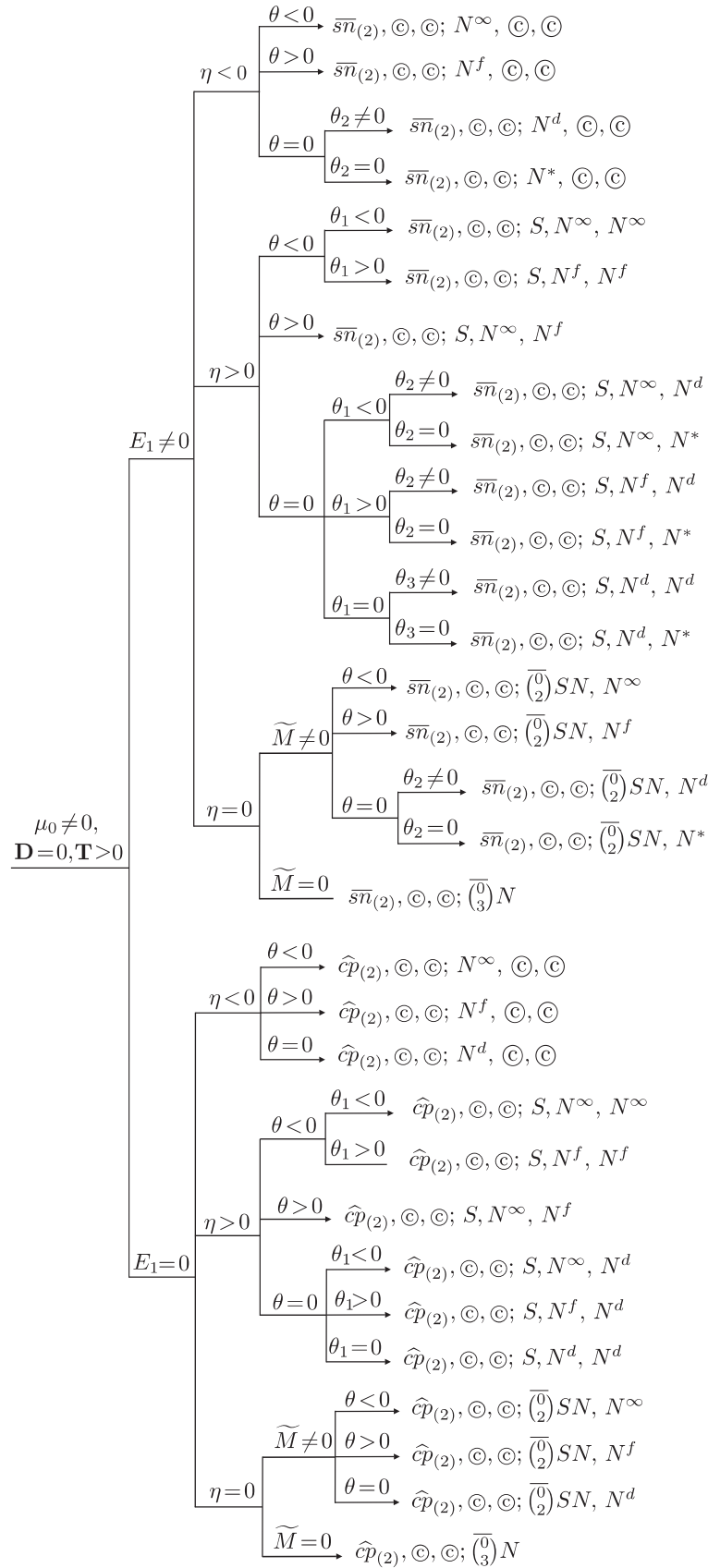
DIAGRAM 1. Global configurations: the case \mu_0 \neq 0, \mathbf{D} = 0, \mathbf{T} > 0 .
