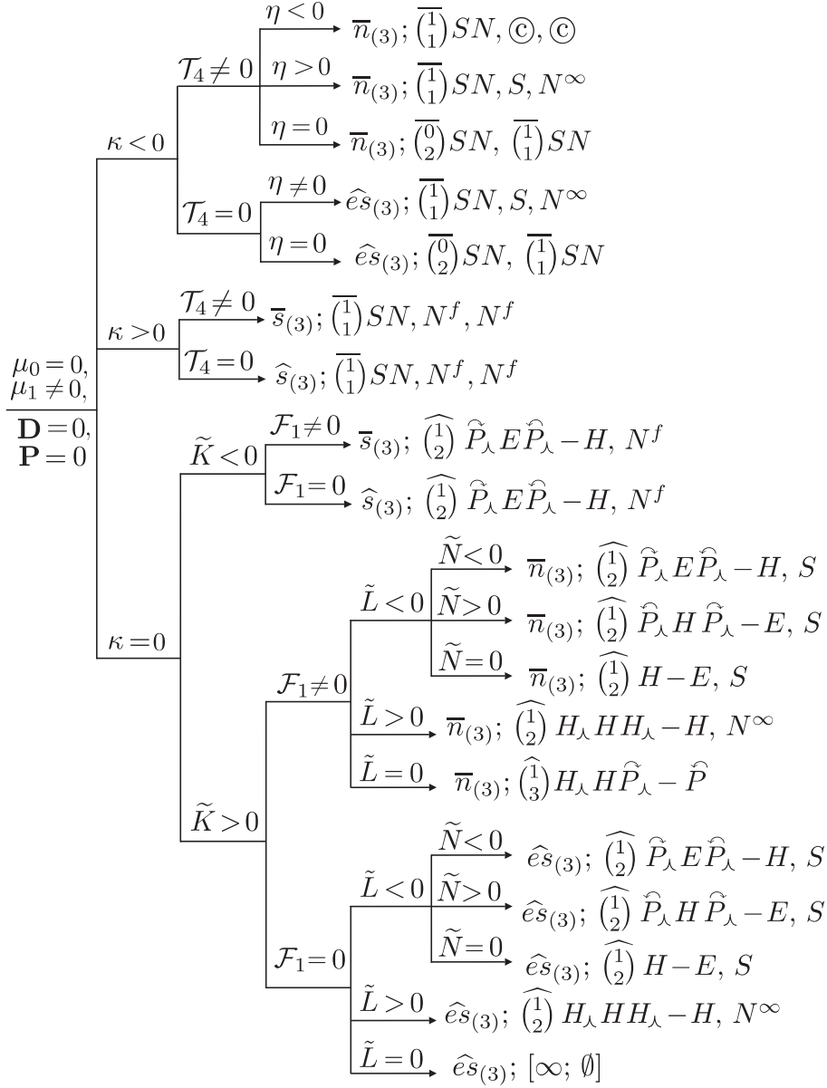
DIAGRAM 3. Global configurations: the case \mu_0 = 0, \mu_1 \neq 0, \mathbf{D} = \mathbf{P} = 0 .
