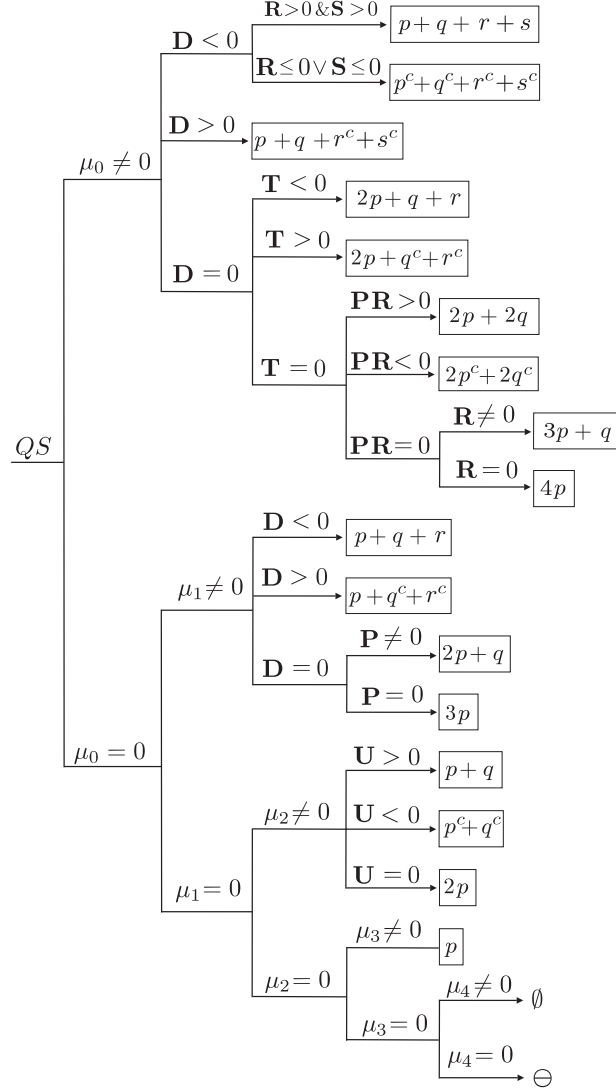
FIGURE 1. Diagram for Finite Singularities of Quadratic systems
