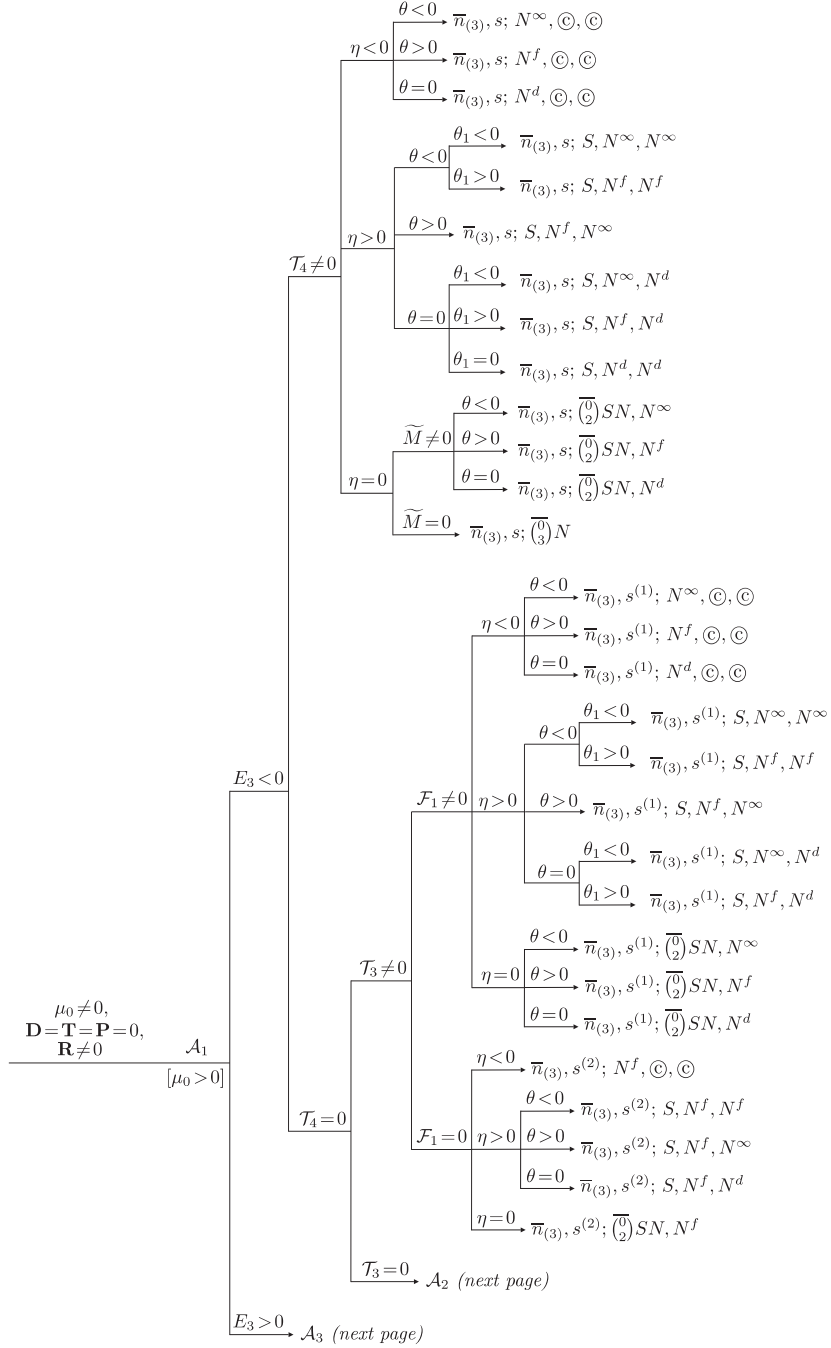
DIAGRAM 3 (continued). Global configurations: the case \mu_0 \neq 0 , \mathbf{D} = \mathbf{T} = \mathbf{P} = 0 , \mathbf{R} \neq 0 .
