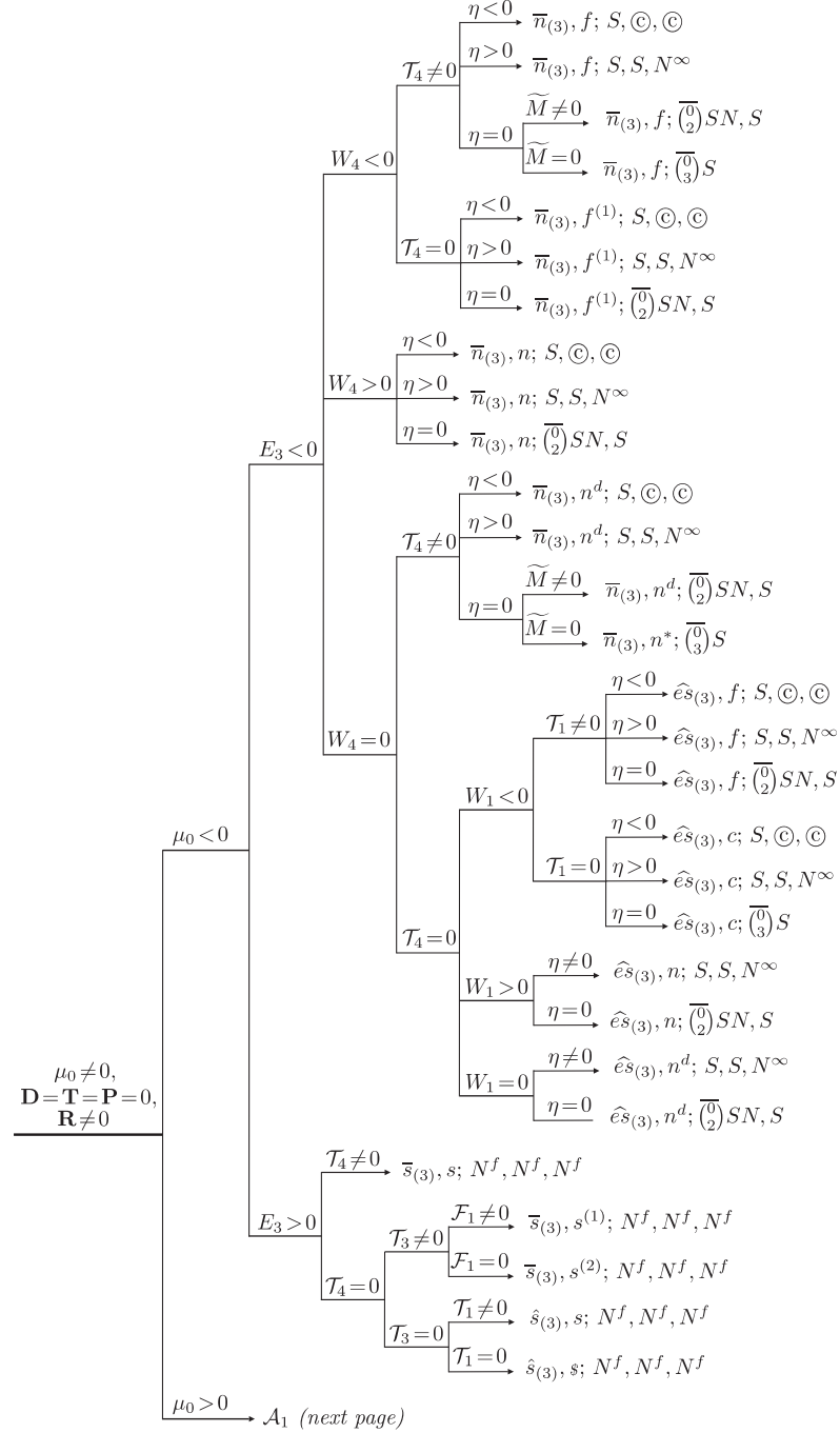
DIAGRAM 3. Global configurations: the case \mu_0 \neq 0, \mathbf{D} = \mathbf{T} = \mathbf{P} = 0, \mathbf{R} \neq 0 .
