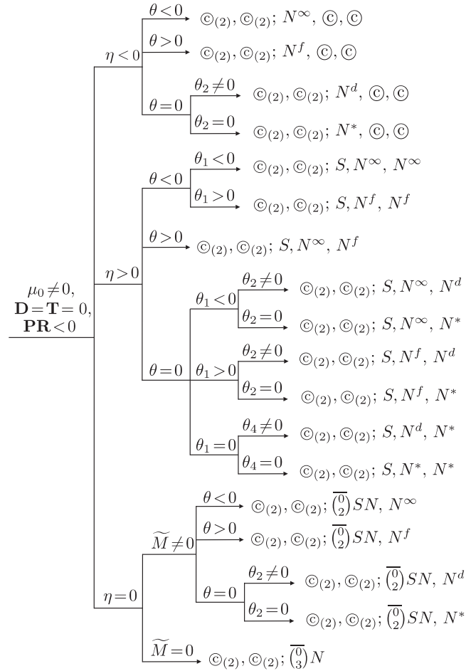
DIAGRAM 1. Global configurations: the case \mu_0 \neq 0, D = T = 0, PR < 0 .
