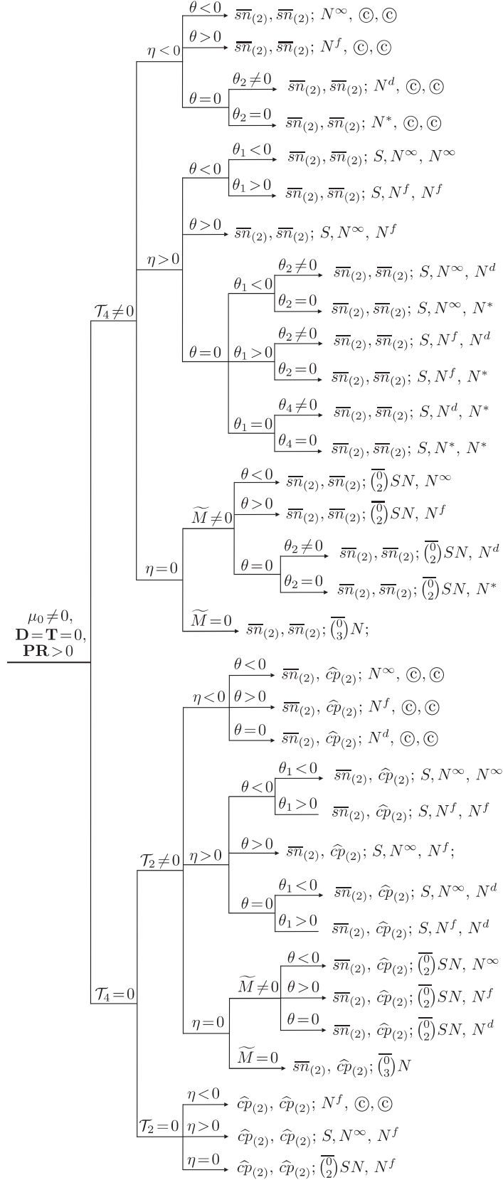
DIAGRAM 2. Global configurations: the case \mu_0 \neq 0 , \mathbf{D} = \mathbf{T} = 0 , \mathbf{PR} > 0 .
