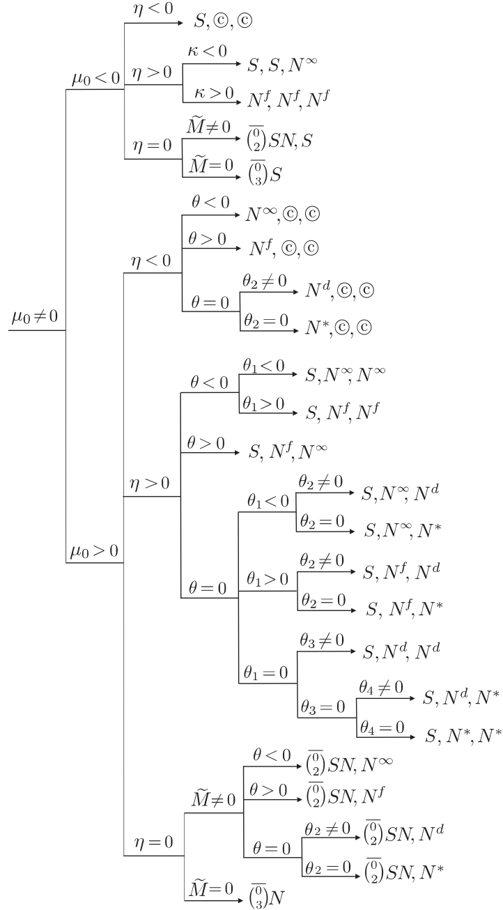
DIAGRAM 4. Configurations of infinite singularities: the case \mu_0 \neq 0 .
