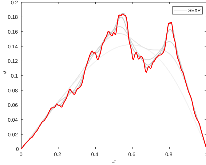
Figure 3: Almost sure convergence of the exponential integrator (SEXP). The reference solution is displayed in red.
