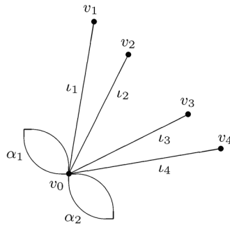
FIGURE 1. The pointed graph (G_2, A_5) .
