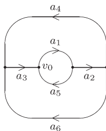
FIGURE 3. The graph G of Example 5.4.
