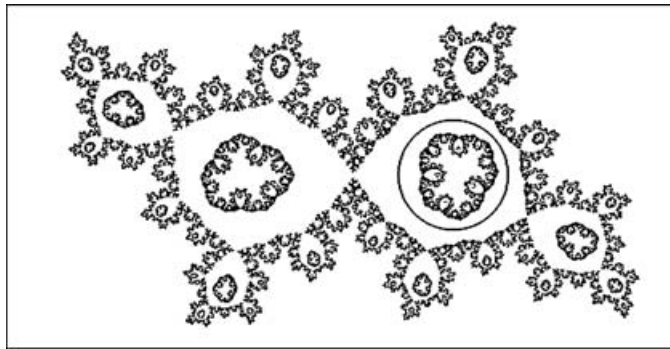
FIGURE 2. For t = 0.615\,173\,215\,88\dots , the rational map f_{e^{2i\pi t}, 1/4} leaves the circle \mathbb{S}^1 invariant and has a Herman ring.
