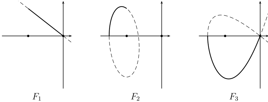
FIGURE 6. The different pieces F_i, i = 1, 2, 3
