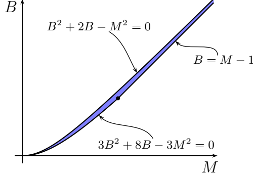
FIGURE 4. Curves that define the region \mathcal{R} (colored), that contains W(M, B) = 0
