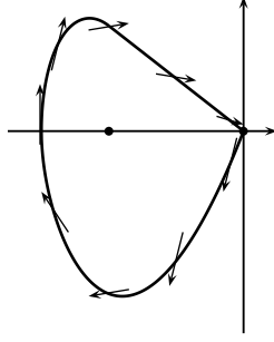
FIGURE 7. The negatively invariant region corresponding to the piecewise loop
