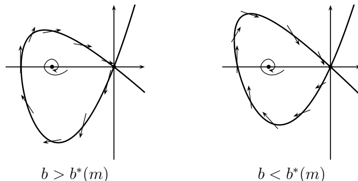
FIGURE 3. Negative and positive invariant regions around the focus
