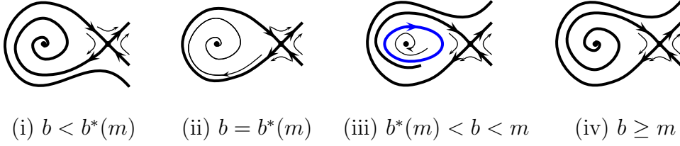
FIGURE 1. Phase portraits of system (1)
