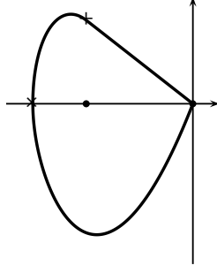
FIGURE 5. Piecewise loop for obtaining a negatively invariant region
