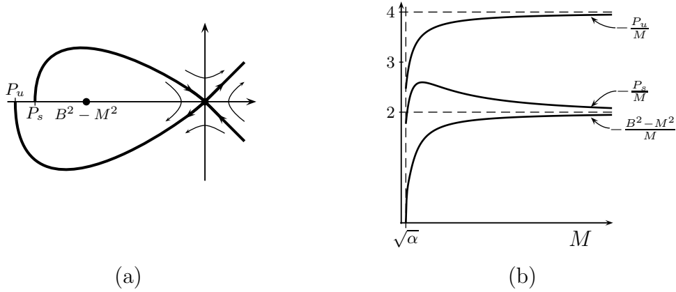
FIGURE 8. Separatrices of the saddle point
