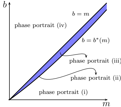
FIGURE 2. Sketch of the bifurcation diagram of system (1). The open colored region is the one containing the limit cycle
