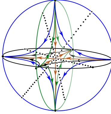
FIGURE 2. Phase portrait of system (1) on the planes x = 0 , y = 0 , z = 0 inside the Poincaré ball.
