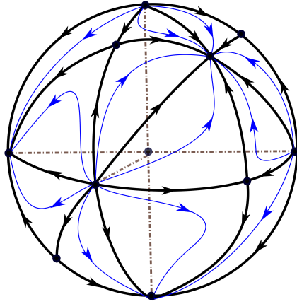
FIGURE 4. Phase portrait of system (1) at infinity on the boundary of the Poincaré ball for x \geq 0 .
