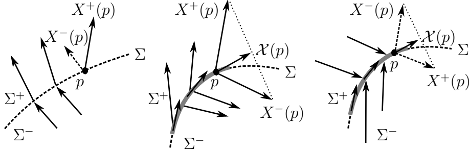
FIGURE 1. Definition of the vector field on \Sigma following Filippov's convention in the sewing, escaping, and sliding regions.
