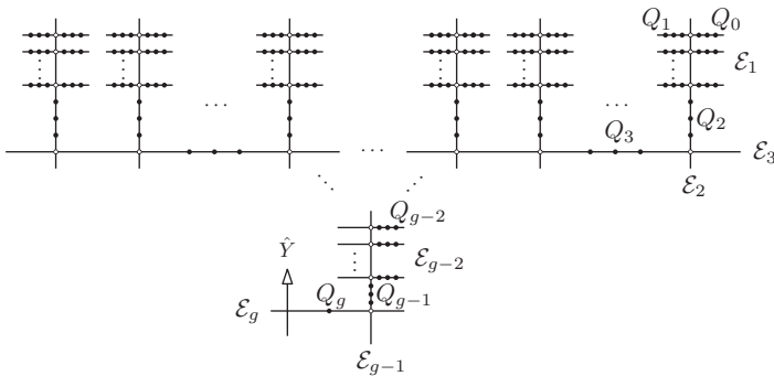
FIGURE 4. Resolution of Y \subset S .
