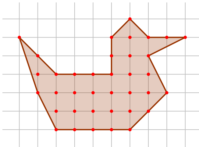
Figura 4: Aquí: F(P) = 21 , I(P) = 16 y A(P) = 16 + \frac{21}{2} - 1 = \frac{51}{2} .
