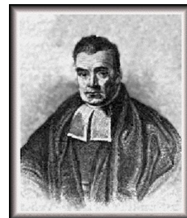
Th. Bayes (1702-1761)
