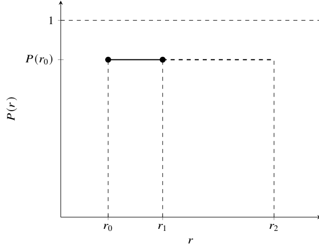
Fig. 1 First, since r_1 > 1/(1 - \sqrt{1 - \varepsilon}) and r_0 = r_1\sqrt{1 - \varepsilon} + 1 , P is constant and equal to P(r_0) on the interval [r_0, r_1] . Then, the same argument shows that P is constant on each interval [r_n, r_{n+1}] for n \geq 0 .
