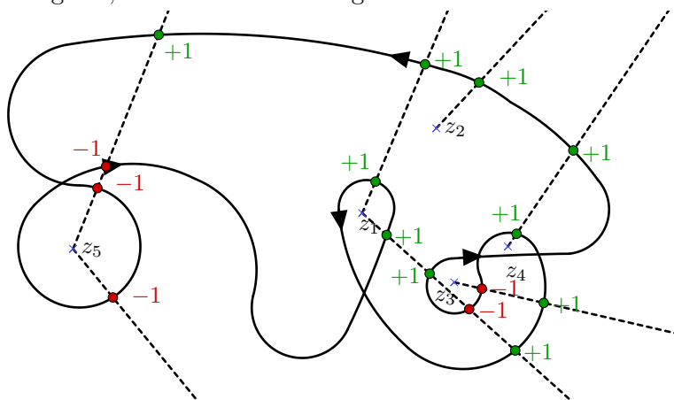
Figura 5.4: Trobem \text{Ind}(\gamma, z_1) = 1 + 1 = 1 + 1 - 1 + 1 = 2 per dues semirectes diferents. Així mateix calculem \text{Ind}(\gamma, z_2) = 1 , \text{Ind}(\gamma, z_3) = 0 , \text{Ind}(\gamma, z_4) = 2 i \text{Ind}(\gamma, z_5) = -1 .
